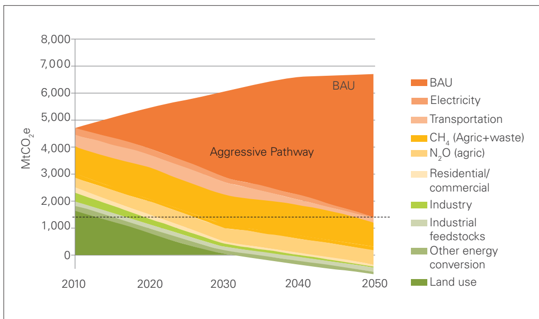
Figure 2.6 Aggressive-I+ Pathway, 2010–50
